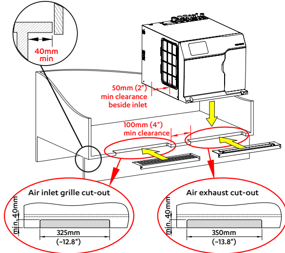
Option 1. Cupboard with 40mm (~1.6") min overhang
