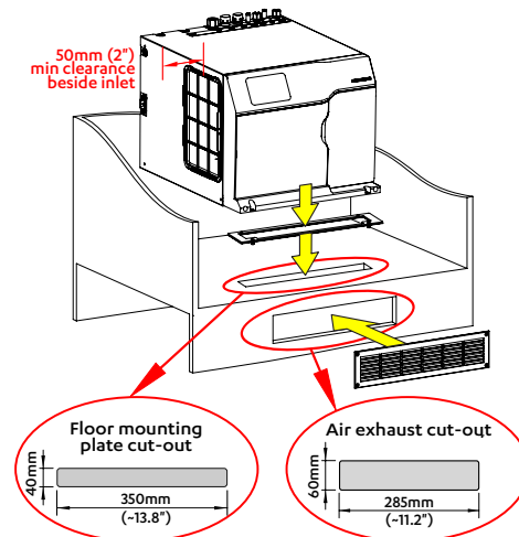
Option 2. Cupboard with less than 40mm (~1.6") overhang
