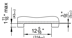
DETAIL B: CABINET FLOOR CUT-OUT
