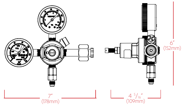
CO 2 Regulator
